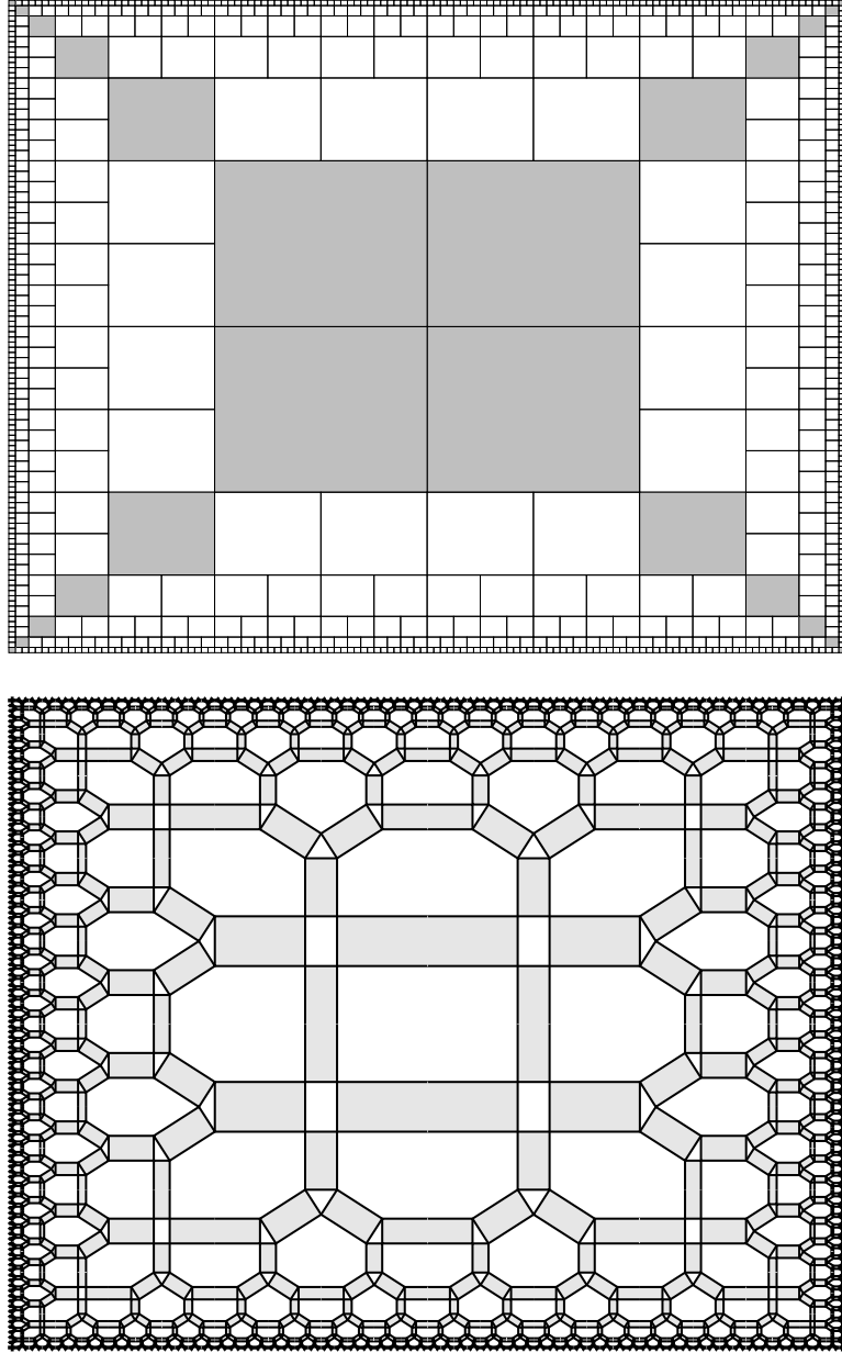
Figure 8: Top. The fractal net of rectangles used to reproduce the singular set of Theorem 5.3. The colored rectangles will host the second module of Figure 7 and the white rectangles will host the first module. Bottom. The resulting singular set \Sigma_u of the map u constructed in Theorem 5.3. The colored rectangles are the regions where \det Du = -1 . Each vertex of the singular set is shared by two rectangles, hence the Kawasaki condition holds.
