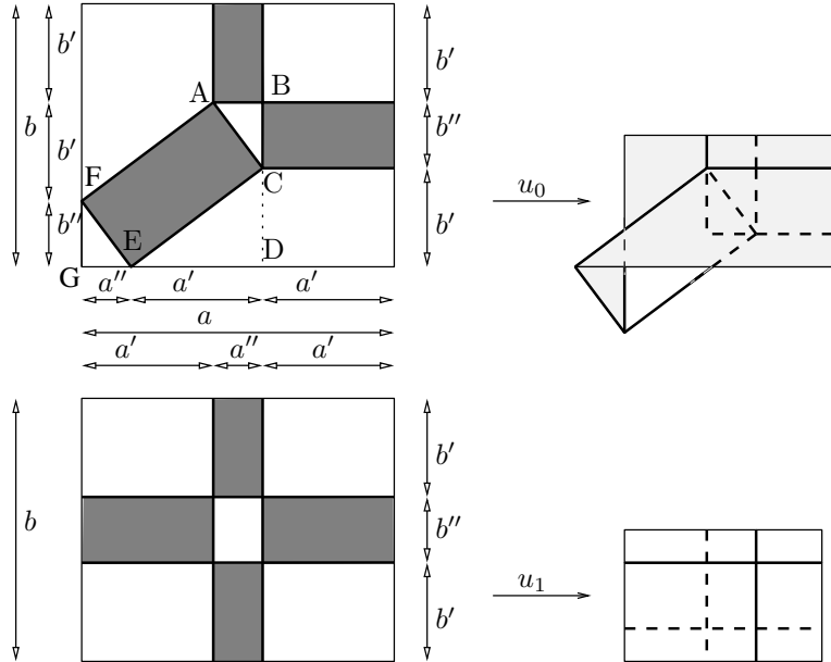
Figure 7: The singular set of the base module used in Lemma 5.2.
