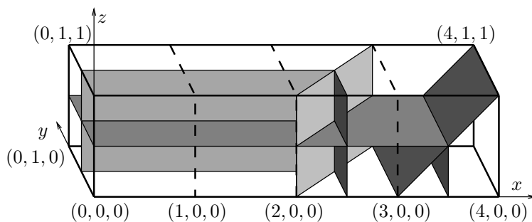
Figure 9: The singular set \Sigma_2 which is the base module of the construction of a 3-dimensional solution to the Dirichlet problem.
