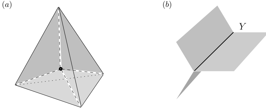
FIGURE 1.1. (a) A soap film spanning the edges of a regular tetrahedron contains four lines of Y -points that share a T -point as their common endpoint at the center of the tetrahedron; (b) the Y -cone consists of three half-spaces meeting along a common boundary line by forming equal angles.
