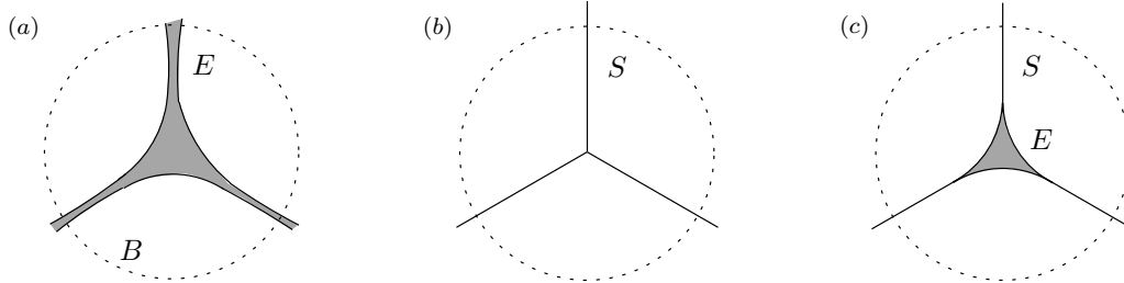
FIGURE 1.2. Three ways of looking at a same soap film: (a) as a three-dimensional region E occupied by a liquid at equilibrium (capillarity theory); (b) as a two-dimensional surface S (the “mid-section” of the three-dimensional region E ) with singularities that obey Plateau’s laws (dry model); (c) as a combination of a two-dimensional surface S and a three-dimensional region E “wetting” the location of Plateau singularities (wet model).
