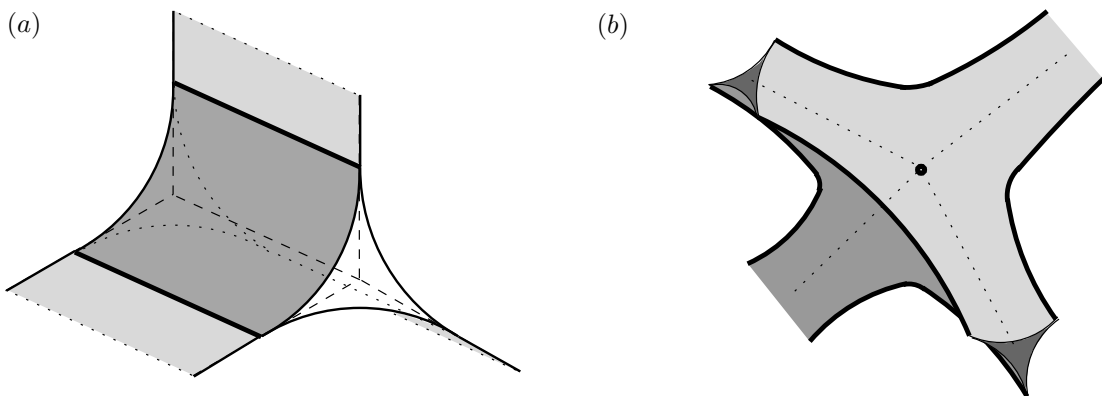
FIGURE 1.3. Plateau borders near Y -points (a) and T -points (b). The transition region between zero and negative mean curvature is assumed to happen along transition lines and with continuity of the unit normal.
