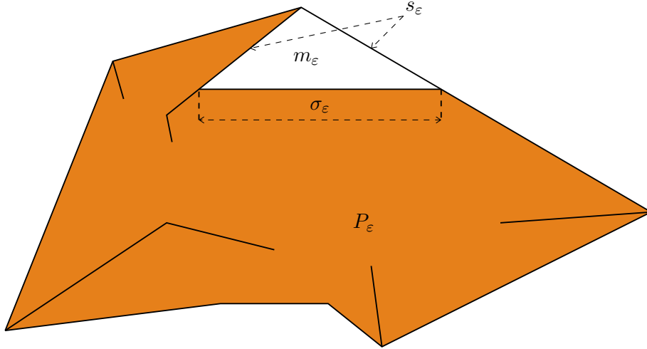
FIGURE 5. The cutting procedure of P
