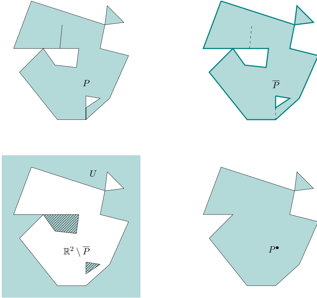
FIGURE 9. Construction of P^\bullet
