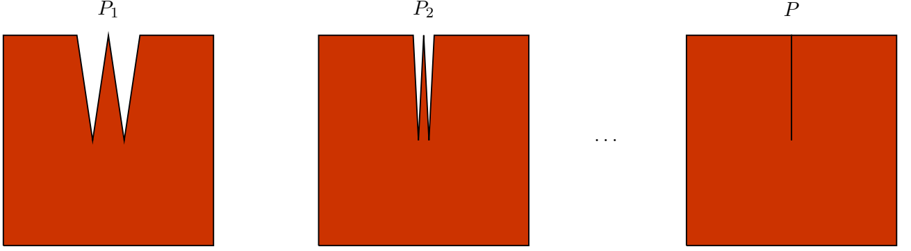
FIGURE 3. \widetilde{Per}(P_n) \rightarrow 12 > 10 = \widetilde{Per}(P) .
