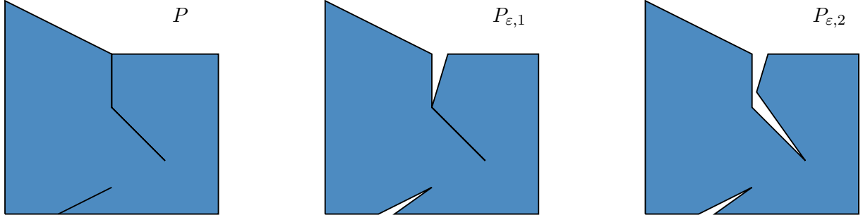
FIGURE 8. When a crack of P consists of more consecutive segments, we apply the procedure several times
