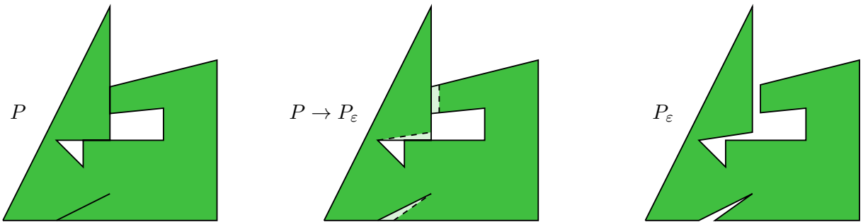
FIGURE 7. Building P_\varepsilon starting from P
