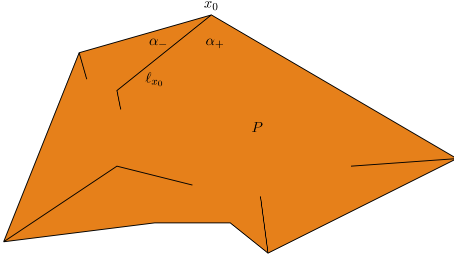
FIGURE 4. In the polygon P all convex corners are determined by self-intersected sides; choosing the vertex x_0 as above, without loss of generality, we can argue only on P \cap \alpha_+ or P \cap \alpha_- .
