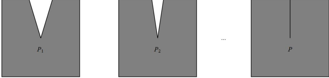
FIGURE 1. The sequence (P_n) \subset \mathcal{P}_7 H^c -converges to the “degenerate polygon” P , which has a boundary given by line segments, but is not a simple polygon.
