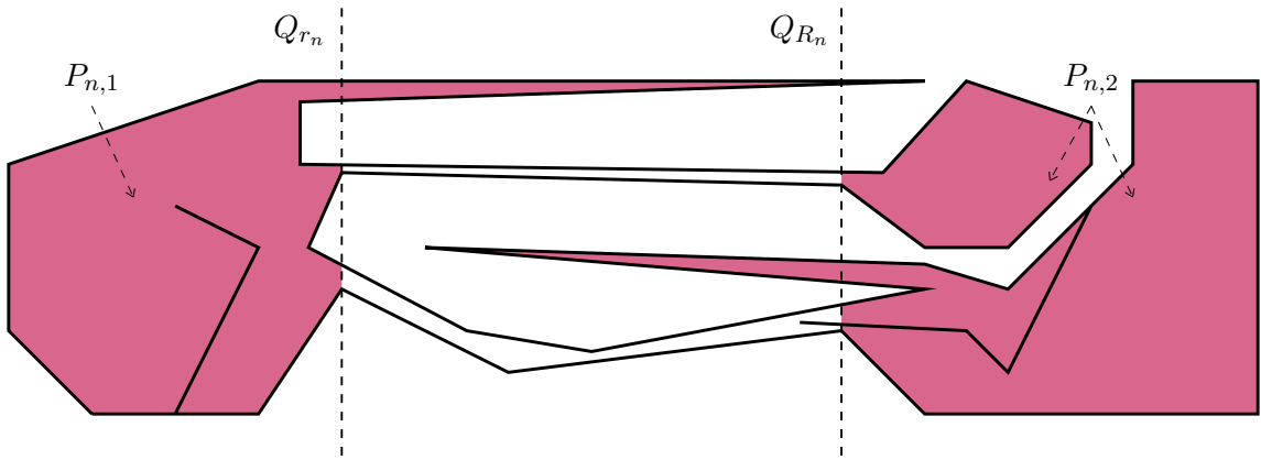
FIGURE 6. P_n is the generalized polygon with the black contour; P_{n,1} and P_{n,2} are detected in color as in the picture.
