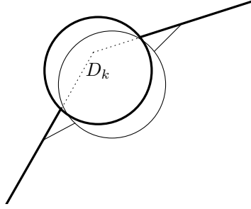
FIGURE 4. If two rays are emitted from a cluster D_k , they should have opposite directions otherwise we could translate D_k in a direction which enables us to decrease the local length of the rays.
