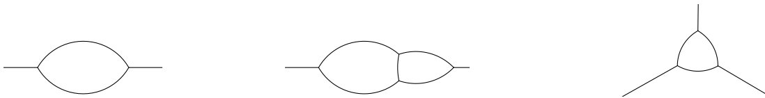
FIGURE 1. The lens, the peanut and the Reuleaux partition.
