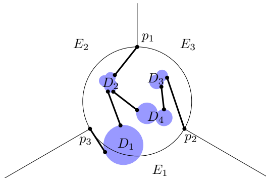
FIGURE 5. The components D_1, \dots, D_4 in the proof of Theorem 4.3 Step 2.
