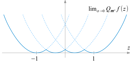
Figure 20: the limit of Q_{m^\sigma} f for \sigma \rightarrow 0 in the case m_1 = 0 .
