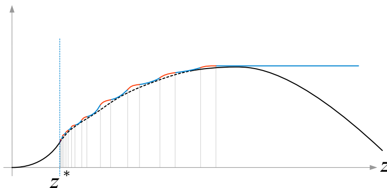
Figure 31: comparison between the graph of the function g_{\text{hom}} (below) and that of Q_{\mathbf{m}}f after subtraction of the quadratic part
