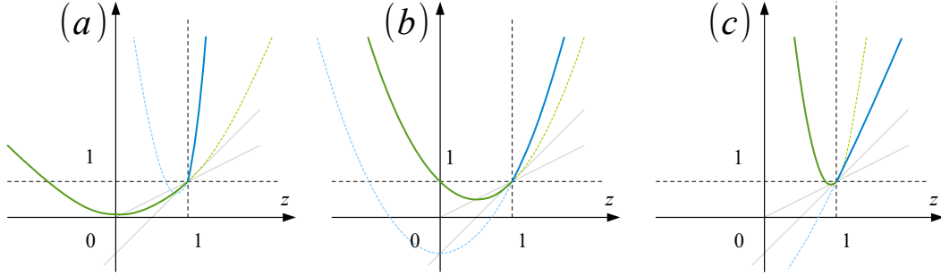
Figure 8: Q_{\mathbf{m}}\ell^\tau(\theta, z) for increasing values of \theta .
