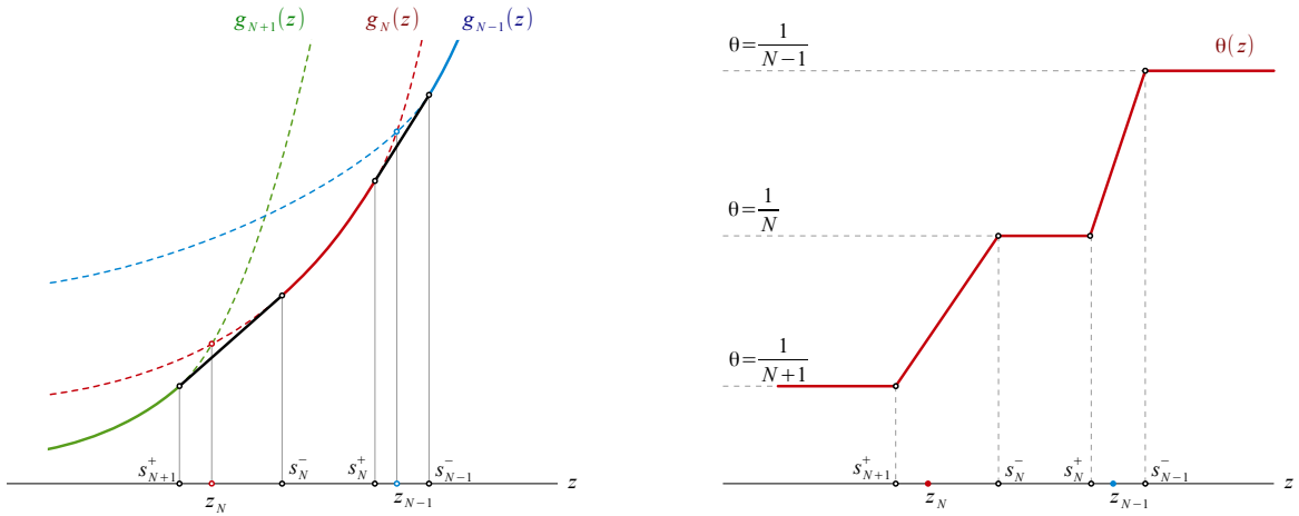
Figure 26: pictorial description of Theorem 5.23 for a single choice of \sigma (shape of \widehat{Q}_\sigma f and \theta , not to scale)
