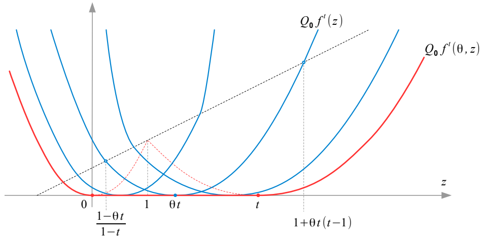
Figure 3: Graph of Q_{\mathbf{0}}f^t(\theta, z) for different values of \theta .
