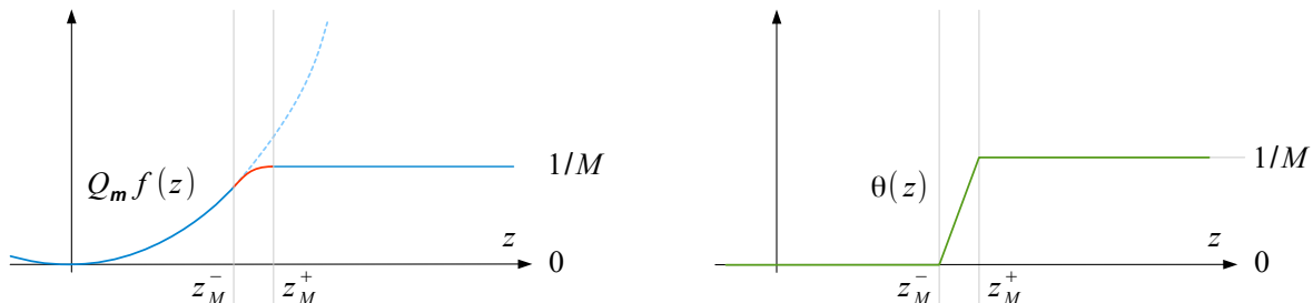
Figure 11: Q_{\mathbf{m}}f and \theta in a degenerate case.
