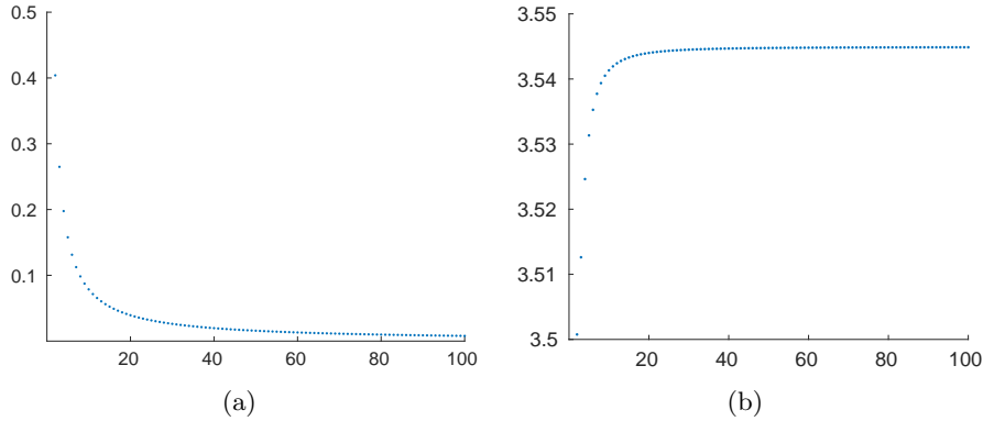
FIGURE 4. Graphs of \bar{x}_n (LHS) and of \mathcal{J}_B[P_n^*] (RHS)
