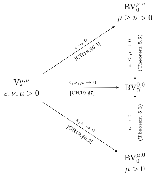
FIGURE 1. The diagram displays the asymptotic relations between different notions of solution. The symbol V_\varepsilon^{\mu,\nu} indicates solutions to the viscous system (1.3). Solid lines represent convergences (along sequences) to the limiting solutions of type BV_0^{\mu,\nu} , BV_0^{\mu,0} , BV_0^{0,0} , already proved in [CR19, Sections 6.1, 6.2, 7]. Dashed lines represent convergences proved in the present paper, the corresponding theorems being referred to in the diagram. Starting from V_\varepsilon^{\mu,\nu} one may either pass to the limit as \varepsilon \downarrow 0 and then as \mu, \nu \downarrow 0 ; or pass to the limit as \varepsilon, \nu \downarrow 0 and then as \mu \downarrow 0 . Since there is no uniqueness, it is not guaranteed that one gets the very same solution found in the joint limit \varepsilon, \mu, \nu \downarrow 0 . However, we prove that through the three different procedures one finds evolutions satisfying the same notion of solution. In this sense we may say that the diagram commutes.
