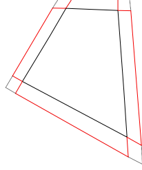
FIGURE 1. Construction of the polygon P_\varepsilon in the proof of Proposition 9
