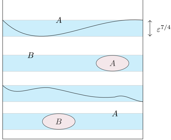
FIGURE 4. A visualization of phase regions in dimension d = 2 . The (anisotropic) second-order penalization guarantees that phase transitions occur inside cylindrical layers of height \varepsilon^{7/4} . (Note that \alpha(d) = 1/4 for d = 2 .) Additionally, \varepsilon^{7/4} is an upper bound on the height of minority islands in the e_2 -direction. In other words, connected components of the phase regions have either small volume or coincide (up to a small set) with a layer of \Omega . In higher dimensions, a similar interpretation is possible, up to higher order terms.
