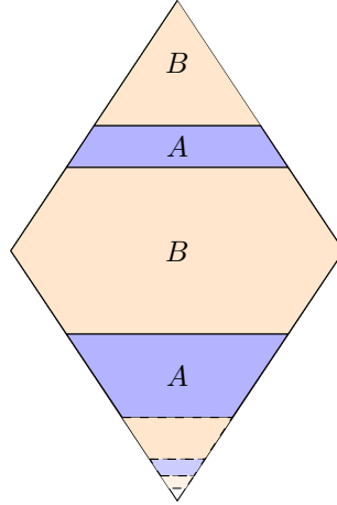
FIGURE 1. The gradient of a limiting deformation y \in \mathcal{Y}_{\text{Id}}(\Omega) , in the case in which B - A = \kappa e_d \otimes e_d .
