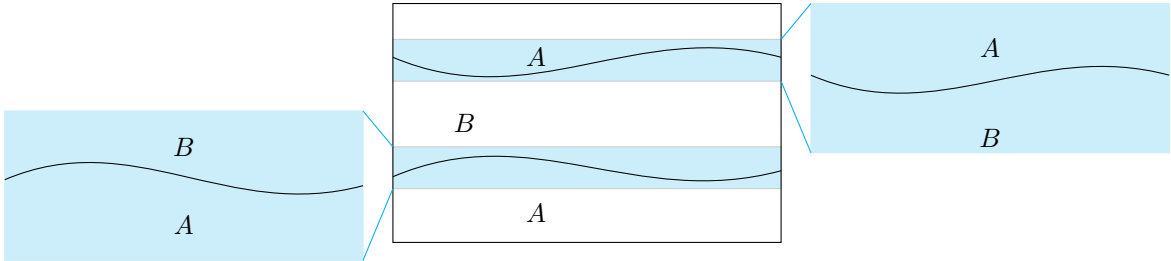
FIGURE 7. By ‘zooming in’ one can identify two regions in which phase transitions occur: the interfaces between the A and B -phase regions become asymptotically flat as i \rightarrow \infty .
