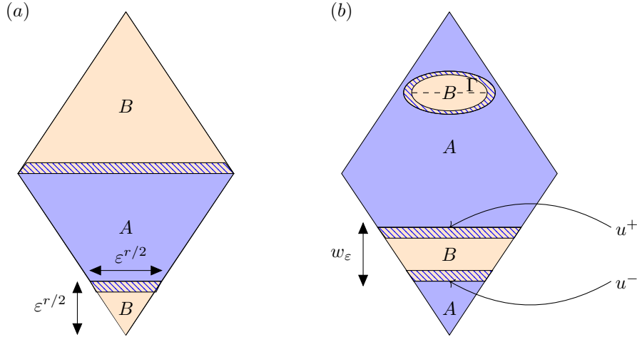
FIGURE 2. (a) Illustration of the A and B phase regions of a deformation y^\varepsilon with finite energy (2.3) in dimension d = 2 . The shadowed regions, where a transition of the gradient between SO(2)A and SO(2)B occurs, are horizontal reflecting the laminate structure of configurations with bounded energy. For the energy (2.8), the phase transition at the lower boundary is possible, whereas the transition in the upper part would lead to unbounded energies as \varepsilon \rightarrow 0 , cf. (2.13). (b) In the upper part of the figure, we depict a minority island centered around a segment \Gamma , which may have length \sim 1 in the e_1 -direction, but width at most \sim \varepsilon , cf. (2.15). Such a set necessarily has curved boundaries and is also penalized by the elastic energy in a neighborhood of the island. In the lower part, the phenomenon described in (2.16) is illustrated.
