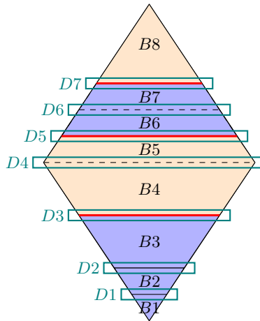
FIGURE 6. A visualization of the different interfaces and sets after the rescaling in Step 1 and under (6.39). The phase regions associated to A and B are colored in blue and orange, respectively. The interfaces associated to the sets \mathcal{I}_y and \mathcal{I}_u are highlighted with thick red and dashed black lines, respectively. The remaining interfaces correspond to the set \mathcal{I}_{\mathcal{P}} . The connected components of \Omega \setminus J_u are indicated as \{B_i\}_{i=1}^8 , whereas the cylindrical sets \{D_i\}_{i=1}^7 around the interfaces (see (6.44)) are drawn in green.
