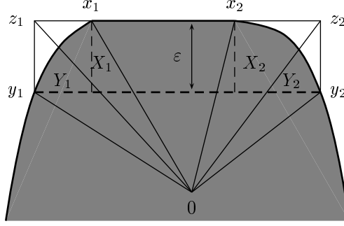
Figure 7: The construction used in Lemma 4.4.
