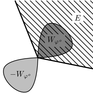
Figure 1: There may be infinite many minimal cones with one component. If W_\varphi has no vertices then these cones are half-planes. In this and in the following pictures translations of W_\varphi are filled with dark gray while translations of -W_\varphi are filled with light gray.
