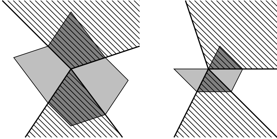
Figure 2: On the left a minimal cone with two components when W_\varphi is a quadrilateral. The only other minimal cone is its complementary set. On the right one of infinitely many minimal cones with two components when W_\varphi is a triangle.
