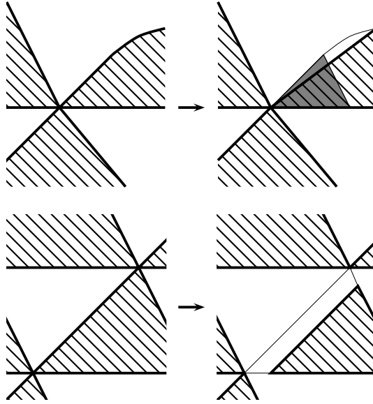
Figure 6: How to lessen the perimeter of E in the proof of Theorem 3.11
