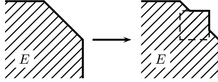
Figure 9: How to increase the volume of E by adding a small square ball.
