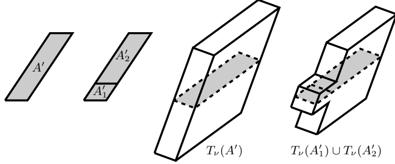
FIGURE 2. An example with N = 2 in which T_\nu(A') \neq T_\nu(A'_1) \cup T_\nu(A'_2) .
