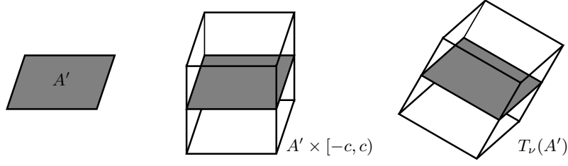
FIGURE 1. Construction of the oriented n -dimensional interval T_\nu(A') .
