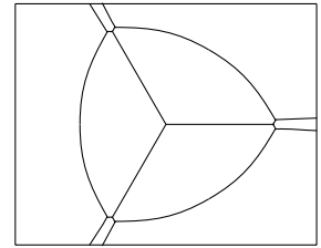
Cisgenerate 3-ray star \Theta = ?
