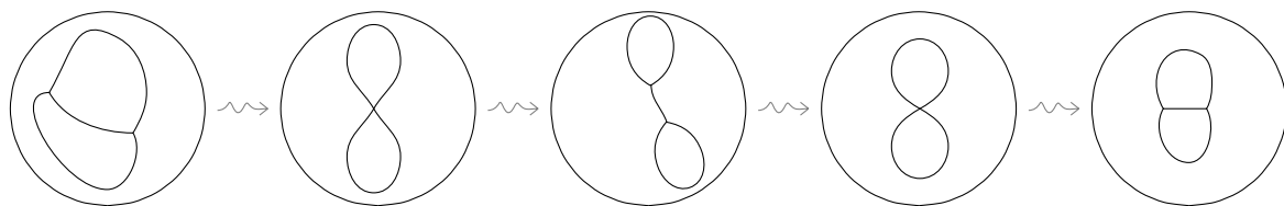
Figure 34: Switching by standard transitions of a \Theta -shaped network to an “eyeglasses-shaped” one and viceversa.
