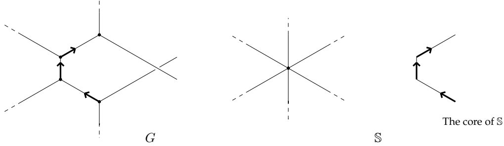
Figure 11: If the assigned unit tangent vector “turns” of an angle of 60 degrees in the same direction for two consecutive times, G has self-intersections. An example of such a pair (G, \mathbb{S}) .
