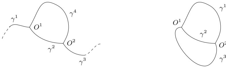
Figure 8: A lens/fish-shaped and a \Theta -shaped network.
