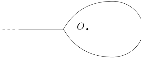
Figure 7: Another example of regular shrinker with one triple junction: a Brakke spoon .
