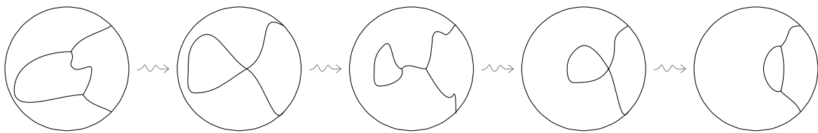
Figure 33: Standard transitions switching a lens-shaped network to an “island-shaped” (with a bridge) one and viceversa.
