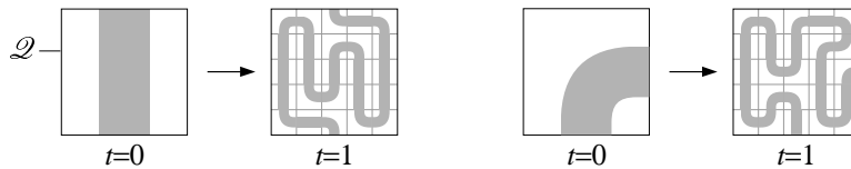
FIGURE 5. An example of basic family for a quasi-self-similar construction: the sets in gray are the supports E_j of the solutions \rho_j for j = 1 (left) and j = 2 (right) and at times t = 0 and t = 1 .
