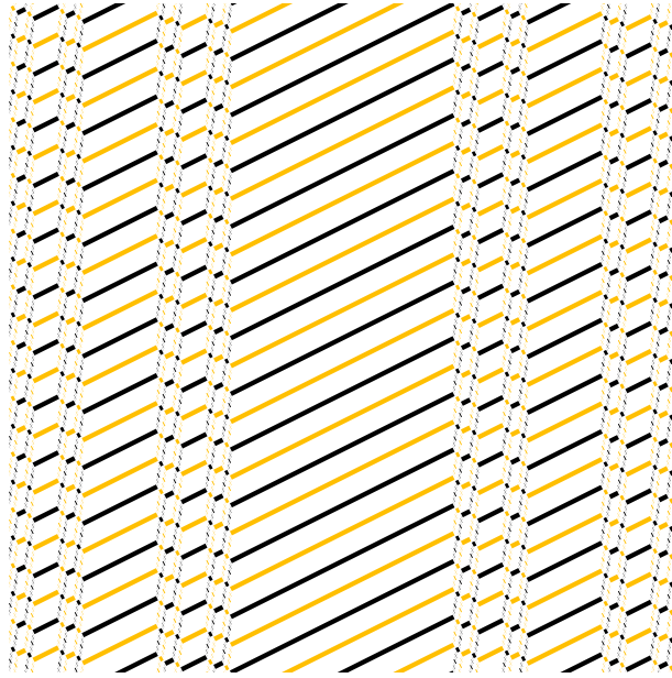
Figure 1: Curves satisfying \dot{\gamma}(s) = 1 almost everywhere may fail to be Lipschitz continuous, this is why characteristic curves are required to be absolutely continuous. Being automatically C^1 -functions, they are then stable under uniform convergence.
