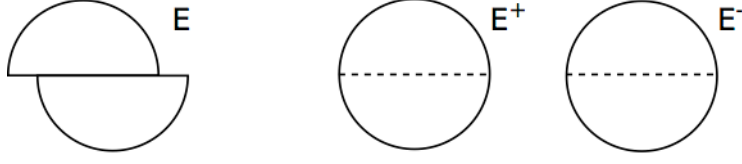
FIGURE 4. Counterexample to (4.20)
