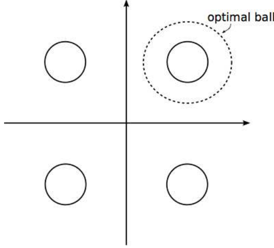
FIGURE 2. The optimal ball of a n -symmetric set is not always centered at the origin
