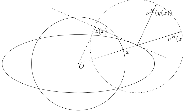
FIGURE 1. The construction in Lemma 3.3
