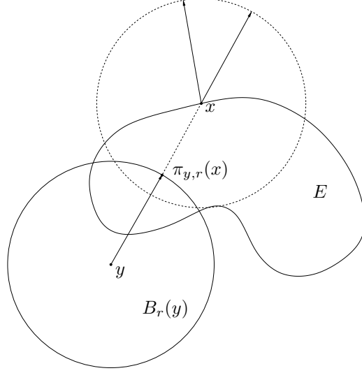
FIGURE 9. The construction of the oscillation index
