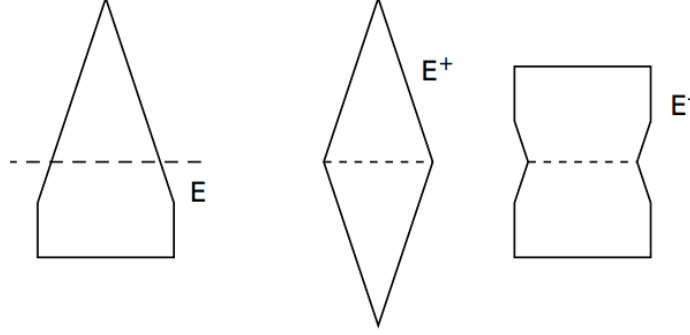
FIGURE 3. Construction of E^+ and E^-
