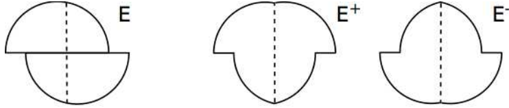
FIGURE 5. A different symmetrization may give a bigger asymmetry
