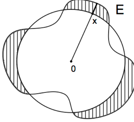
FIGURE 6. |E\Delta B_1| \leq C \int_{\partial^* E} |1 - |x||
