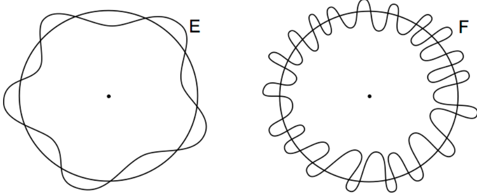
FIGURE 8. E and F have the same measure and the same asymmetry
