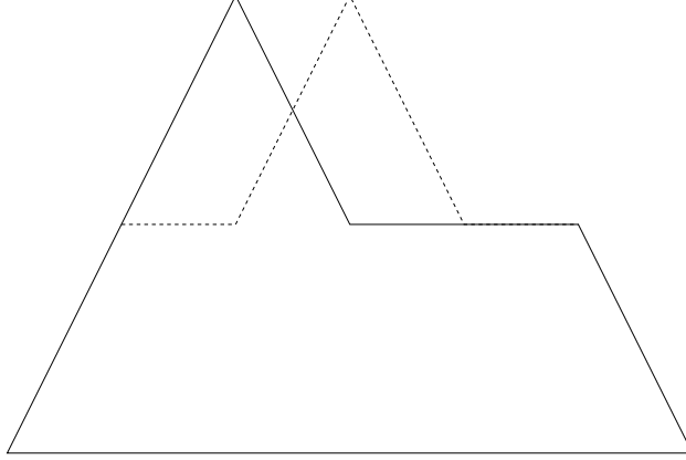
FIGURE 10. An example showing the necessity of condition (6.16) to deduce that f is a translated of f^*
