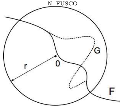
FIGURE 7. A perimeter almost minimizer F
