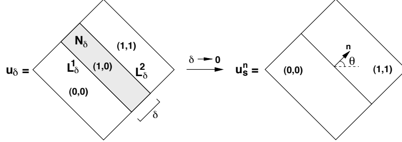
FIGURE 2. Splitting the jumps is energetically favorable
