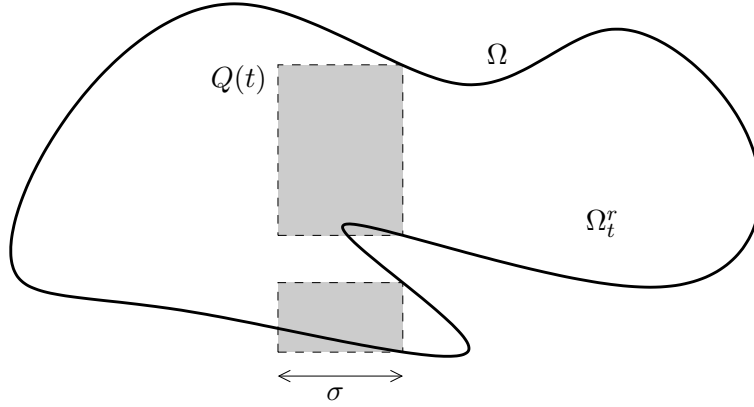
FIGURE 1. A set \Omega with the cylinder Q(t) (shaded).
