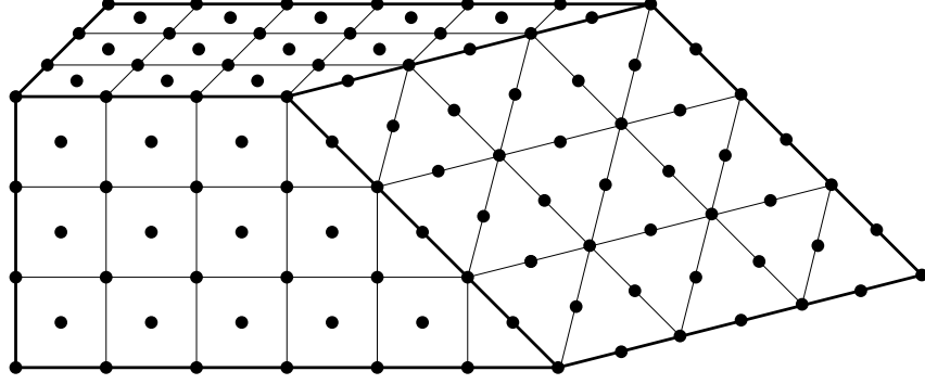
FIGURE 14. By cutting the face-centred cubic lattice on a certain transverse plane, one obtains a two-dimensional hexagonal Bravais lattice. Notice that the lines indicate the geometry of the setting and not the bonds between nearest neighbours.
