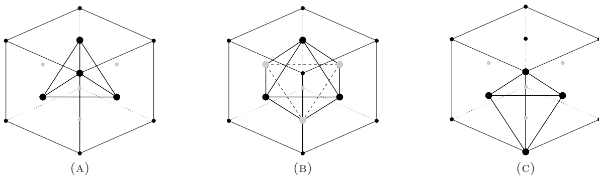
FIGURE 13. Unit cell of the face-centred cubic lattice: the nearest-neighbour structure of the atoms provides a subdivision of the space into tetrahedra and octahedra. (A) tetrahedron; (B) octahedron; (C) quarter of octahedron. Grey dots denote points lying on the hidden facets.
