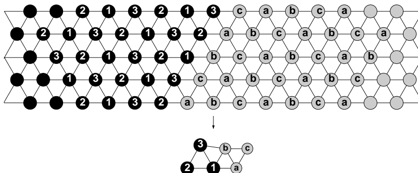
FIGURE 11. A deformation that violates the non-interpenetration condition and maps the lattice \mathcal{L}_{1,\varepsilon}(k) to a configuration consisting of six points. More precisely, all points labelled with the same number or the same letter in the upper part of the figure are mapped to the same point.
