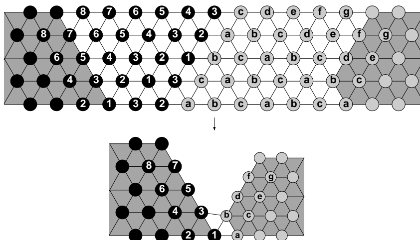
FIGURE 12. If the non-interpenetration condition is neglected, by suitably choosing \varepsilon = \varepsilon(k) it is possible to define a sequence of deformations \{u_\varepsilon(k)\} of \mathcal{L}_{1,\varepsilon}(k) such that u_\varepsilon(k) gives the equilibrium away from the interface and the total interaction energy \mathcal{E}_\varepsilon^\lambda(u_\varepsilon(k), 1, k) grows linearly in k .
