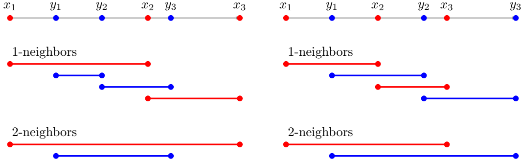
FIGURE 3.1. The figure shows the coordinates of x, y \in \mathbb{R}^3 in two different situations; in particular, in the second case the coordinates of x and y are chosen to make x and y well ordered. In both cases, the sets of 1-neighbors V^1(x) \cup V^1(y) and 2-neighbors V^2(x) \cup V^2(y) are represented, drawing a segment between the endpoints of each couple of neighboring coordinates, in red if the couple belongs to x (namely in V^1(x) or V^2(x) ), in blue if it belongs to y (namely in V^1(y) or V^2(y) ).
