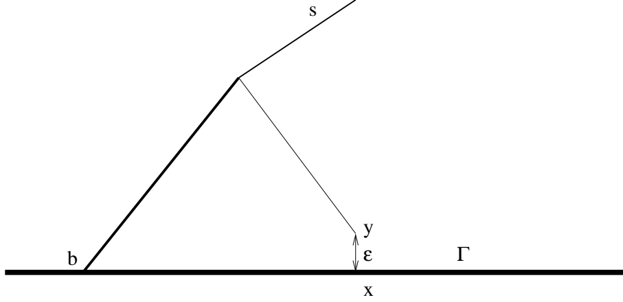
Figure 17: Interpolating-Configuration( \varepsilon, l_{\text{res}} ) (Definition 6.12)
