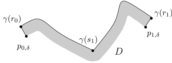
FIGURE 4.2. The situation in Lemma 4.3.
