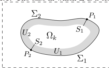
FIGURE 4.1. The case in which \Sigma is a closed curve.
