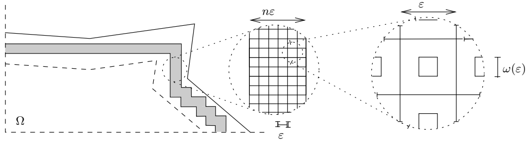
FIGURE 5.5. The construction in Step 3. The set D_{k,\varepsilon} is represented in the picture as the set \Sigma(\delta) \cap \Omega after removing the colored squares contained in the shaded region.
