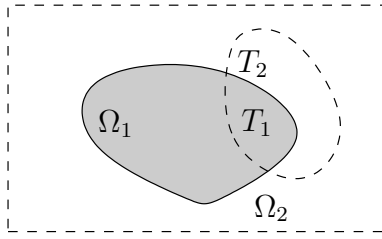
FIGURE 6.2. The dashed line is the contour of the damaged region D .
