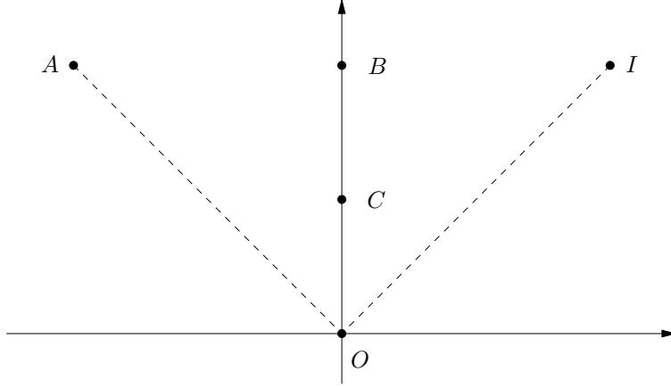
FIGURE 1. A representation of the matrices O , I , A , B and C in \mathbb{R}^2 , identified with the set of the diagonal matrices.
