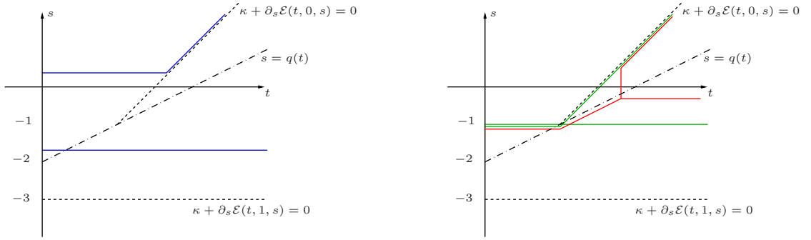
Figure 4.2: Graph of local energetic solutions. More precisely, in the figure on the left, the blue lines correspond to local energetic solutions with initial condition s_0 > -1 and s_0 < -1 . In the figure on the right, we depicted some solutions starting from s_0 = -1 .
