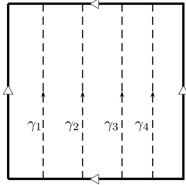
FIGURE 5.1. An example of path on the torus.
