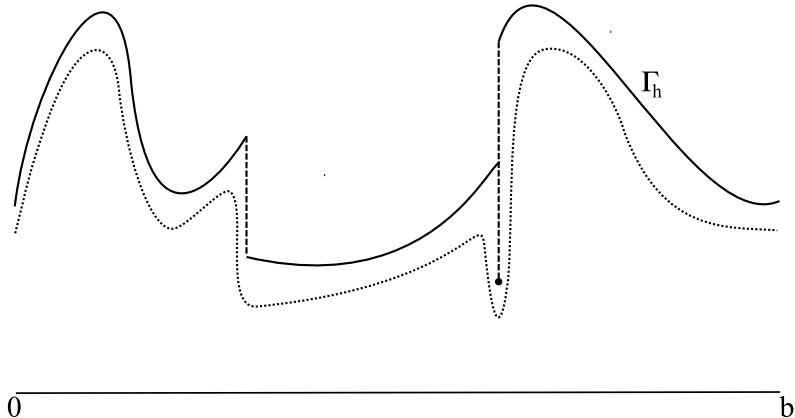
FIGURE 1. An irregular profile h and a smooth approximation. The smooth profile surrounds the vertical cut so that in the limit its length is counted twice.
