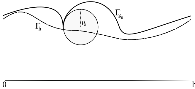
FIGURE 3. If \Gamma_{g_n} contains a cusp or a vertical crack, then, due to the inner ball condition, the L^\infty -distance between g_n and h is comparable to \rho_0 , a contradiction to (1.5).
