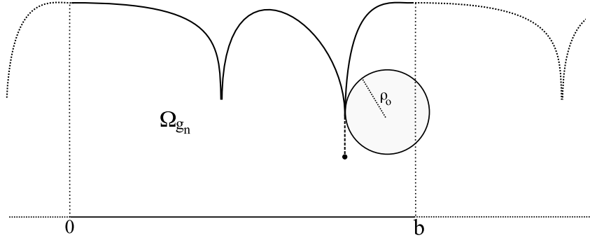
FIGURE 2. The uniform inner ball condition: for each point of \Gamma_{g_n} there is a tangent ball of radius \rho_0 contained in \Omega_{g_n}^\# .
