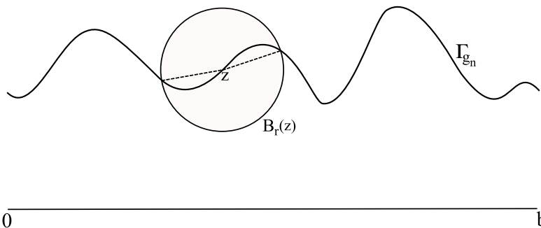
FIGURE 4. The dashed line indicates the profile of the modified configuration used as a competitor to deduce the C^{1,\alpha} uniform bounds.
