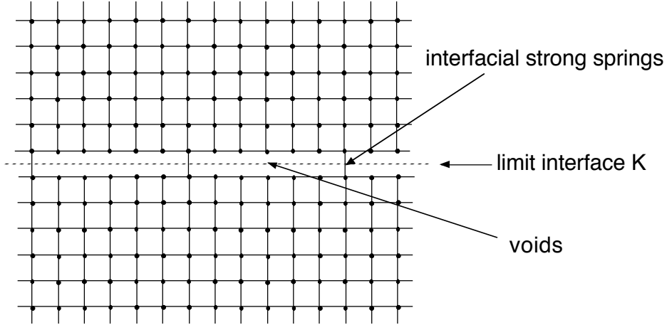
Figure 3: The discrete Neumann sieve
