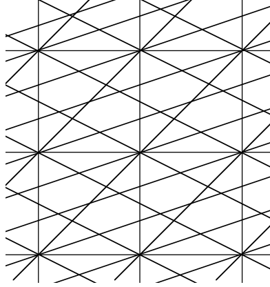
Figure 7: A system of hyperplanes
