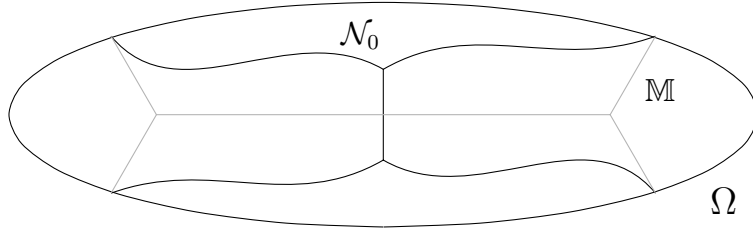
Figure 7: The networks \mathcal{N}_0 and \mathbb{M} .
