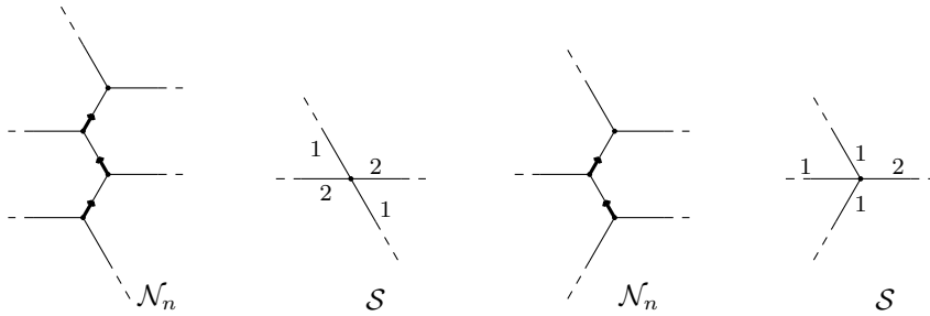
Figure 3: Examples of the edges at the initial/final points of the longest simple path in \mathcal{N}_n and of the relative curves in S , the numbers 1 and 2 denote their multiplicity.
