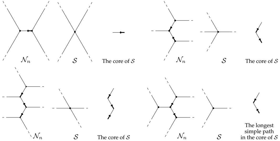
Figure 4: The possible local structure of the graphs G , with relative networks \mathcal{S} and cores, for N = 2, 3, 4 .
