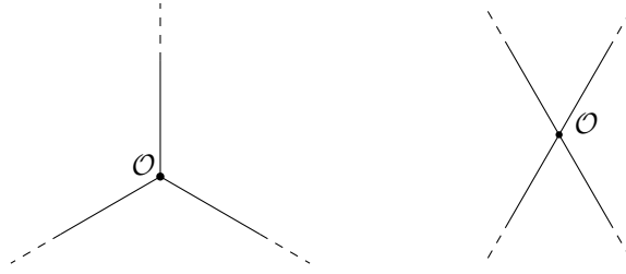
Figure 1: A standard triod and a standard cross.
