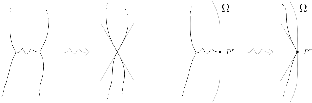
Figure 6: Collapse of a curve in the interior and at an end-point of \mathcal{N}_t .
