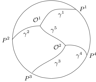
Figure 5: A tree-like network with five curves.
