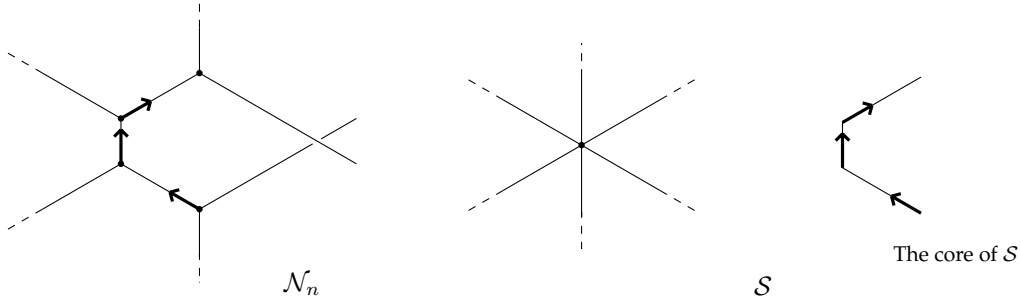
Figure 2: If the unit tangent vector turns of an angle of 60 degrees in the same direction for two consecutive times, \mathcal{N}_n has self-intersections.
