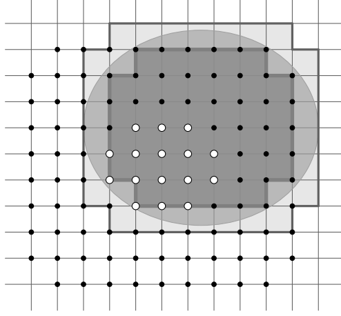
FIGURE 2. We represent some notation used in Section 1. We choose M = 3 . The domain \Omega is the open region contained inside the ellipse, displayed in grey. In light grey the (closed) set \Omega_\eta ; recall that \mathcal{L}_\eta consists of all lattice points in \Omega_\eta . In dark grey the (closed) set \Omega_\eta^b ; points in \mathcal{L}_\eta^b are represented by white dots. Recall that \mathcal{L}_\eta^b \subset \mathcal{L}_\eta^M . The points of \mathcal{L}_\eta^M \setminus \mathcal{L}_\eta^b are represented by black dots.
