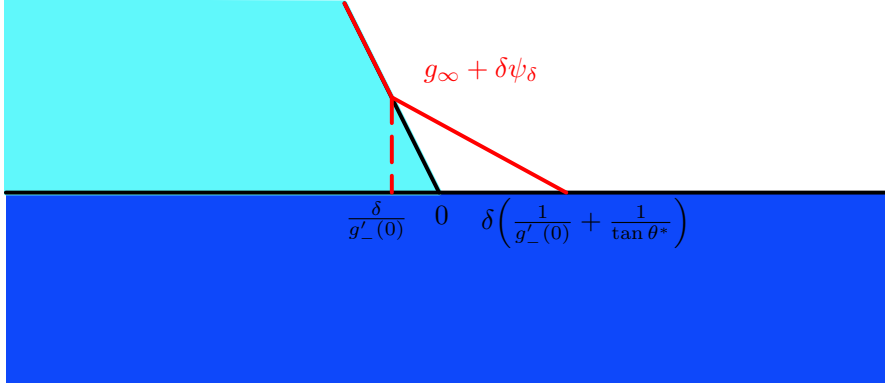
FIGURE 8. The blow-up at island borders (and at valleys with one vanishing contact angle) is displayed. The profile of g_\infty and the perturbation g_\infty + \delta\psi_\delta in the case \theta \geq \theta^* = \arccos \beta for island borders are highlighted in black and in red, respectively
