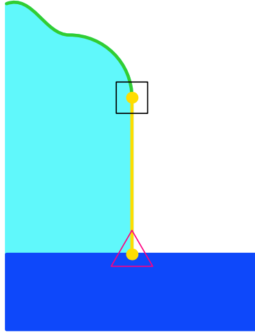
FIGURE 5. Example of a jump at an island border (here indicated with a pink triangle). This is the only type of jump allowed by Theorem 2.3 and only if \min\{\gamma_f, \gamma_s - \gamma_{fs}\}/\gamma_f = 0 .
