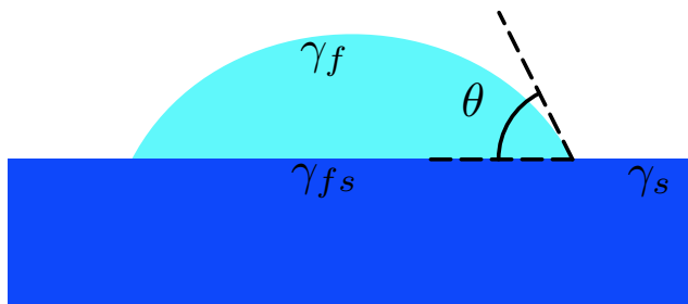
FIGURE 1. Contact angle of a sessile drop.
