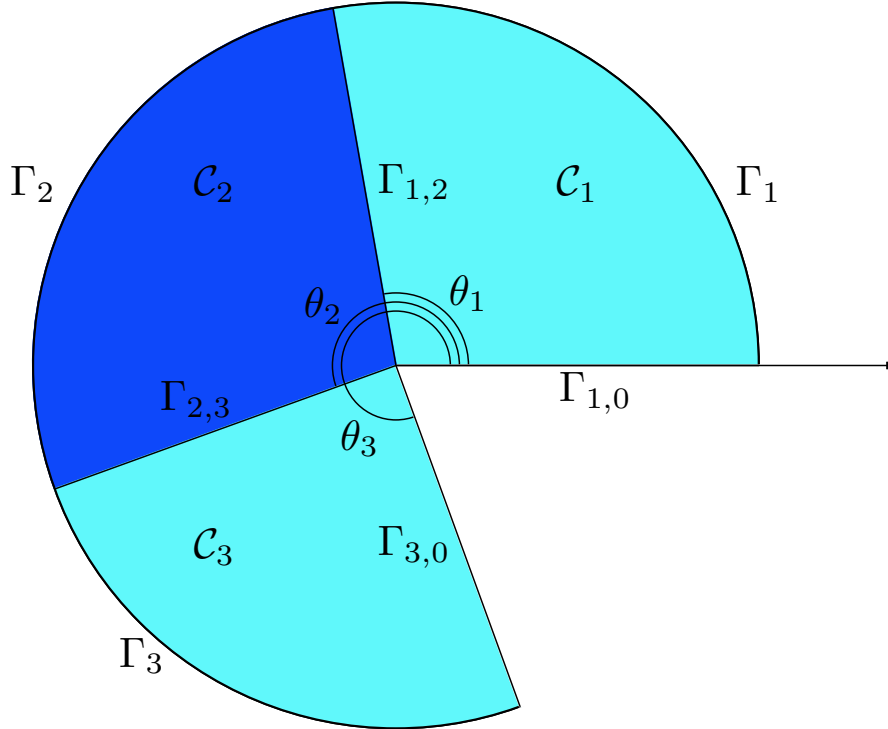
FIGURE 7. The geometry of the set \mathcal{C} on which we consider the transmission problem of Proposition 3.5 is depicted. The lines \Gamma_{1,2} and \Gamma_{2,3} are transmission interfaces for such problem.
