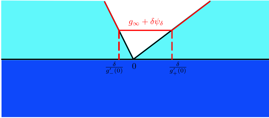
FIGURE 9. The blow-up at a valley with no vanishing contact angle is displayed. The profile of g_\infty and the perturbation g_\infty + \delta\psi_\delta are highlighted in black and in red, respectively
