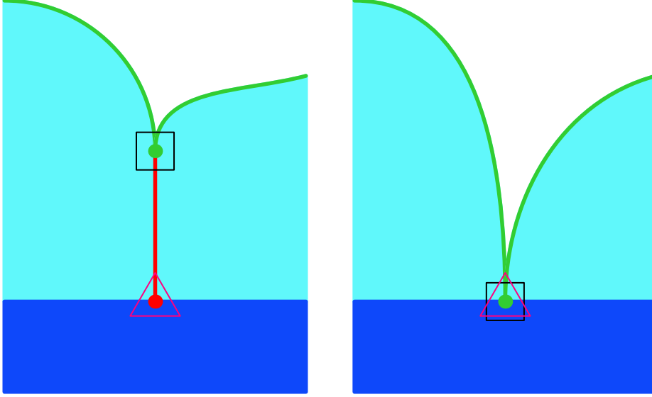
FIGURE 6. Cuts (left) and cusps (right) may represent dislocations at the film/substrate interface.
