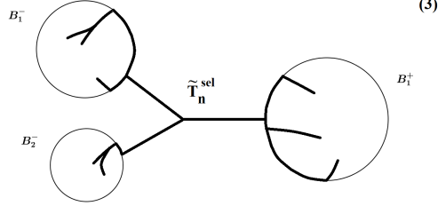
FIGURE 3. The energy competitor \tilde{T}_n^{sel} .
