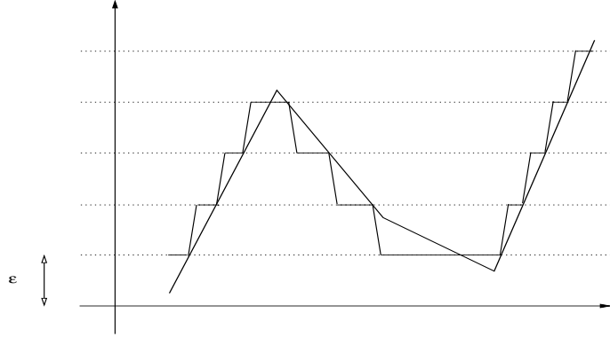
Figure 1: u is represented by the thick line, u_\varepsilon by the thinner one.
