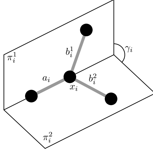
FIGURE 3. The dihedral potential employed in AMBER depends at every atom x_i on the corresponding angle \gamma_i shown in the picture.
