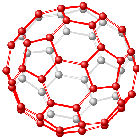
FIGURE 1. The geometry of C_{60} . The bonds shared by two hexagons are here indicated by double lines.
