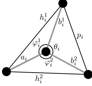
FIGURE 2. Angles, bonds (thick gray lines), and second neighbors (thin black lines) at an atom x'_i \in \mathcal{P}(X_{a,b}) .
