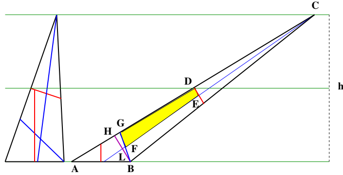
Fig. 3 The heart of a triangle.
