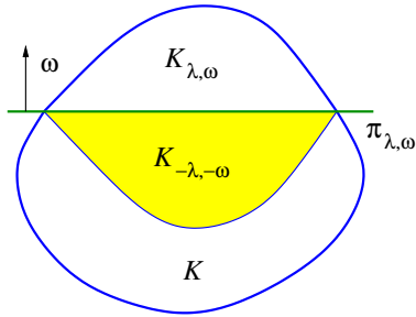
Fig. 1 The sets \mathcal{K}_{\lambda, \omega} and \mathcal{K}_{-\lambda, -\omega} .
